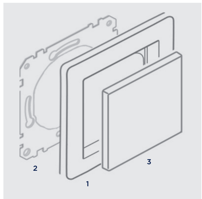
Figure 1. Front plate, frame and adaptor plate
